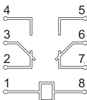
NJX12/2Z
