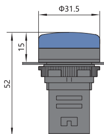
ND16-22DS
