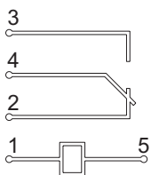
NJX12/1Z
