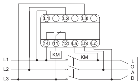
NJYB3-18
