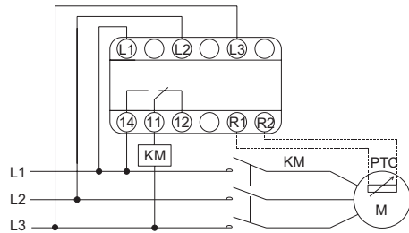
NJYB3-8P, NJYB3-17P
