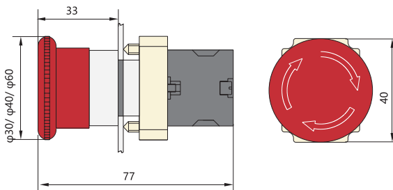
NP2-BS
